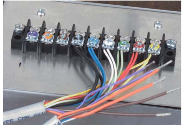
Cable connected to terminal screws
